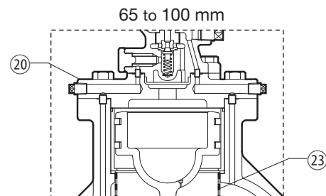
The parts configuration of sizes 65 to 100 mm differs slightly from that of sizes 15 to 50 mm.
